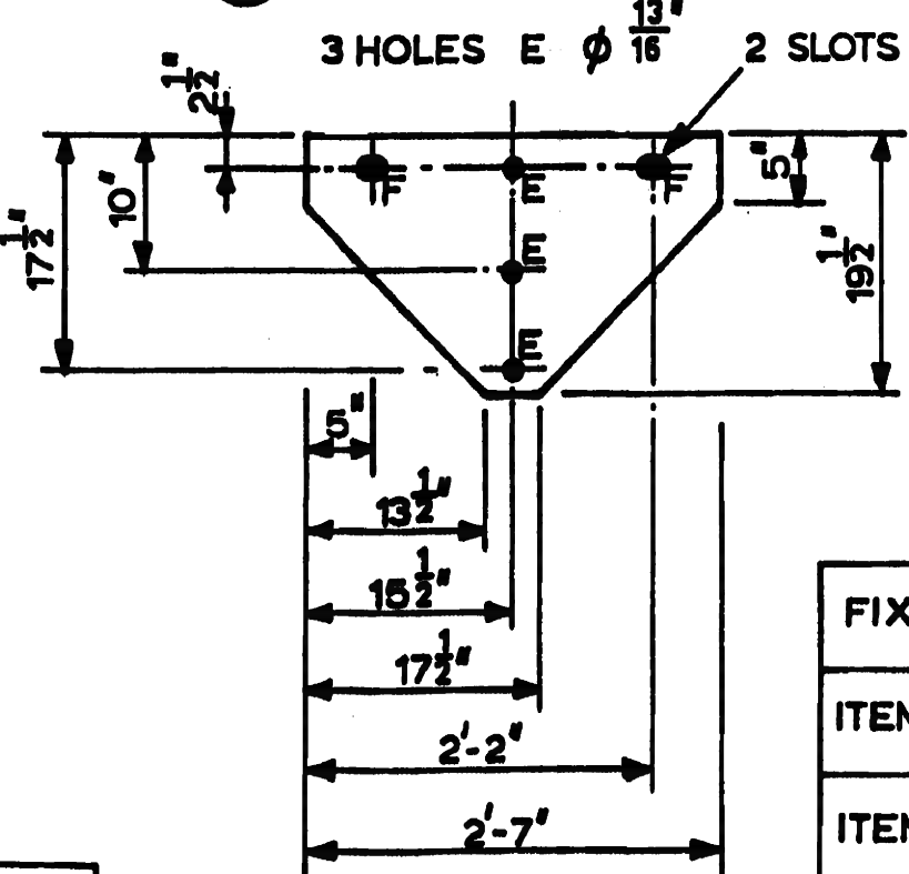
ELEVATION ITEM ③
